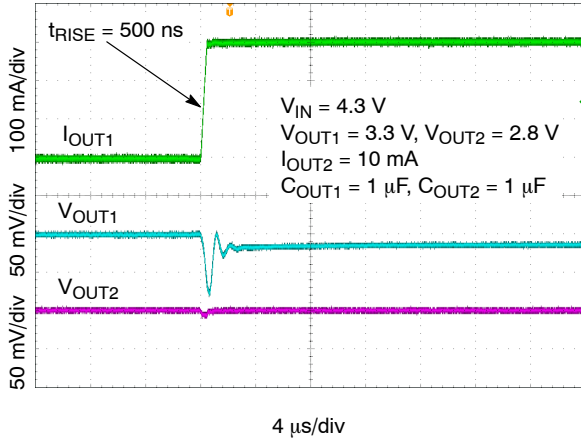
Figure 48. Load Transient Response – 3.3 V – Rising Edge, I_{OUT1} = 1 \text{ mA} to 300 mA
